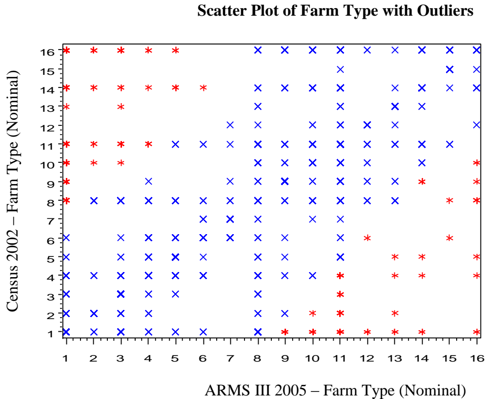
Figures A31-A32: Census 2002 versus ARMS III 2005 Farm Type
