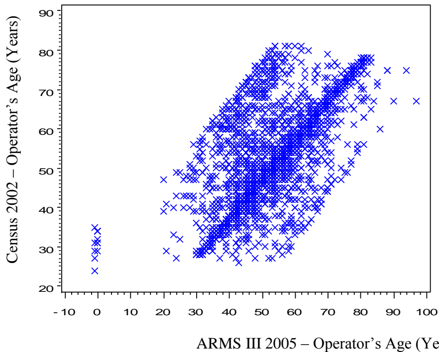
Scatter Plot of Operator's Age without Outliers
